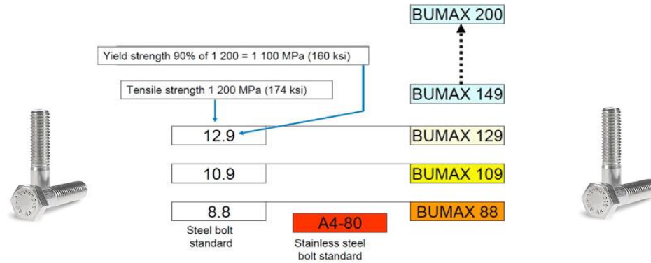
BUMAX High Tensile Stainless Steel Comparison Chart
